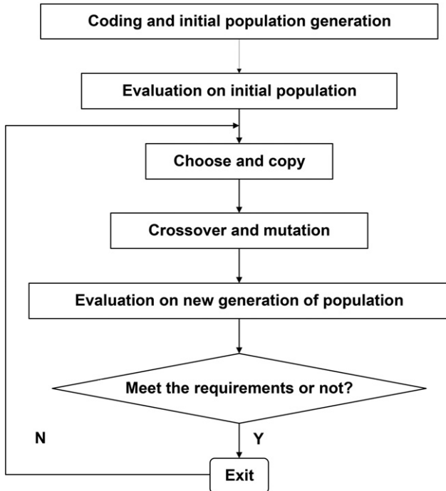
Fig. 5 Genetic algorithm flow.
