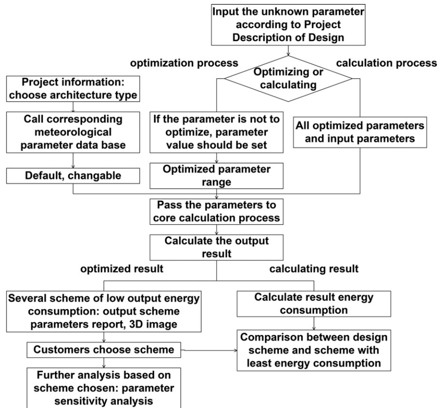
Fig. 7 Software workflow.
