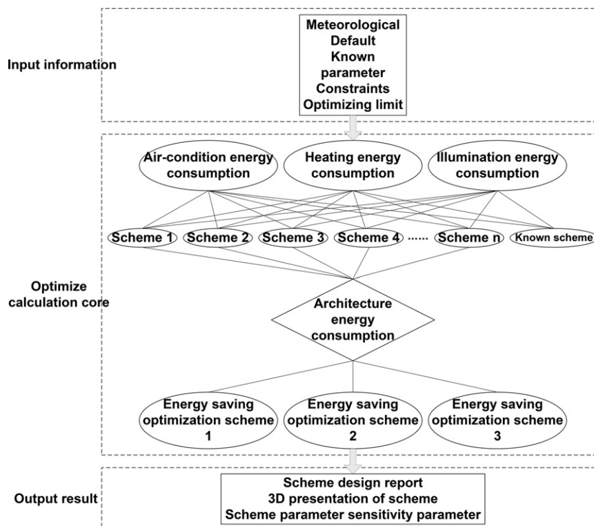
Fig. 8 Software structure.
